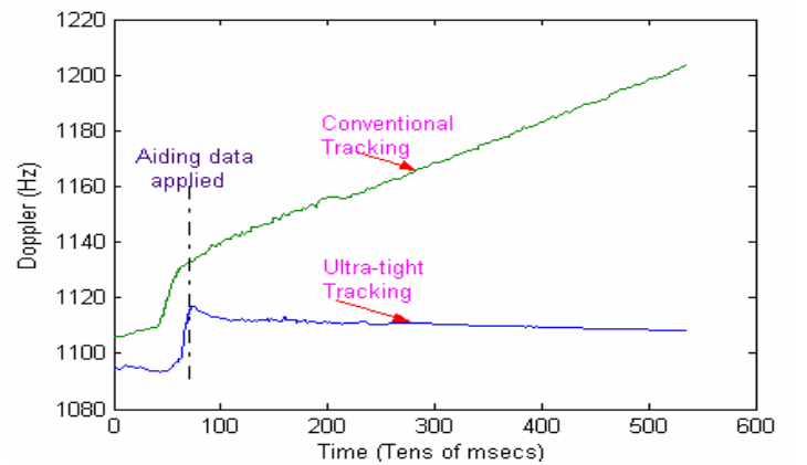
Fig. 3. Conventional vs. ultra-tight carrier tracking loop performance
